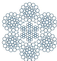
6 x36WS-AACI WS 1-7-7*7-14
